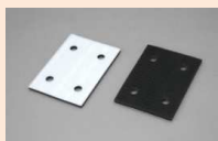
■ Cushion Pad 72mmWx106mmLx5mmT Code: 5535
