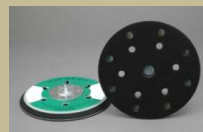
■ Glue-on Pad "D" 148mm dia. x 10mm T. (15 holes) Code: 5573
